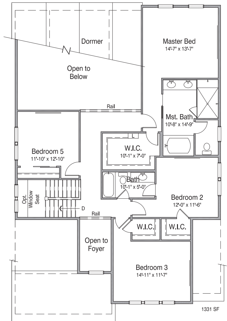
Second Floor
