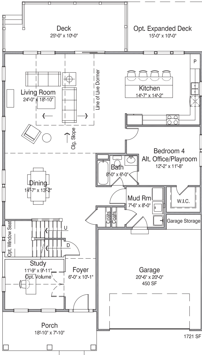
Main Floor
