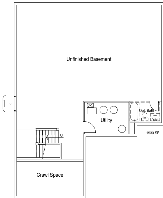
Basement Plan
